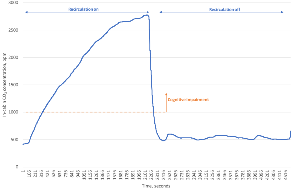
Figure 2: CO 2 build-up with recirculation mode on and off
